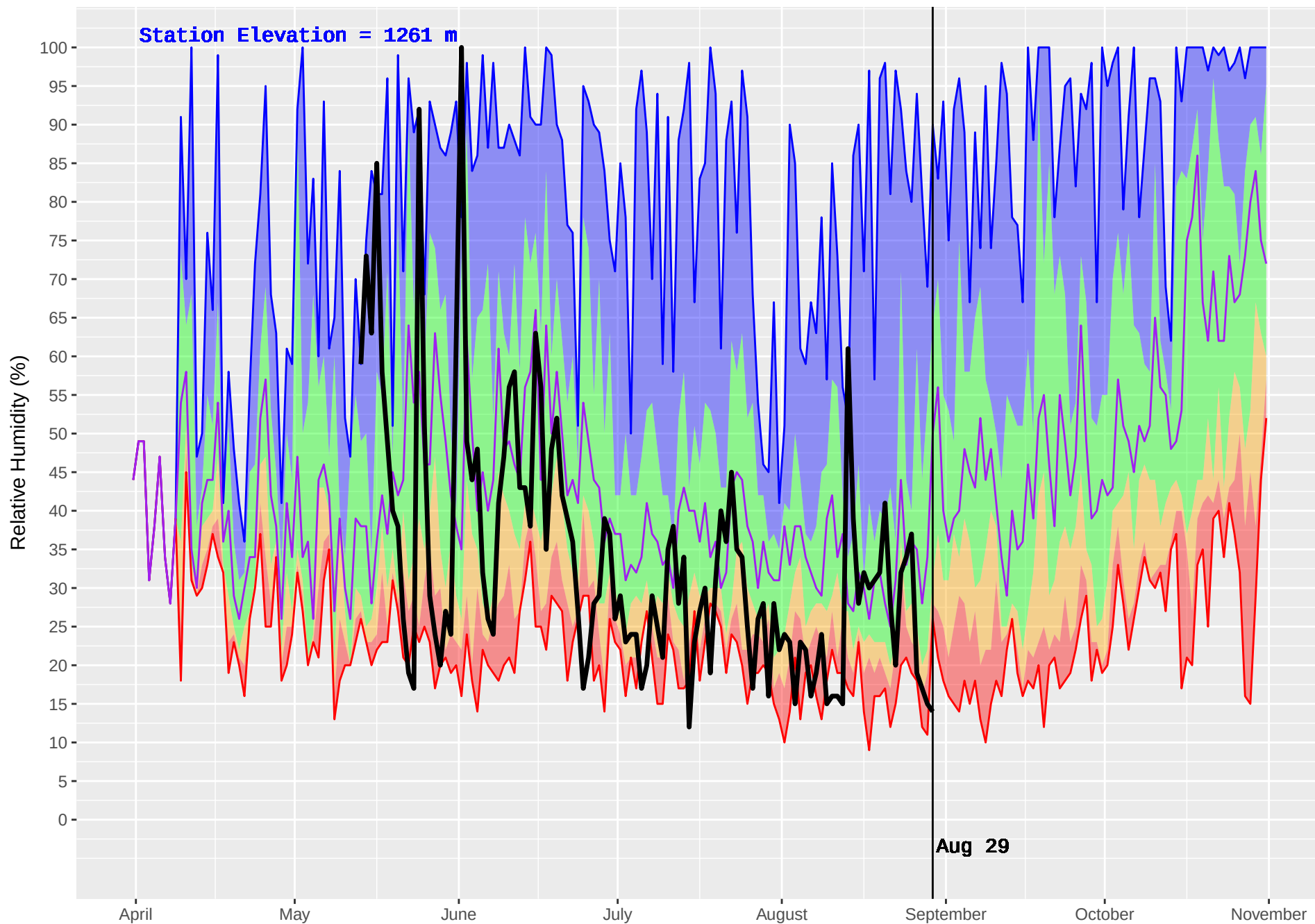
IDA BELL LAKE 3 (876) : Historical (2004–2016) and Current (2017) Noon Relative Humidity
