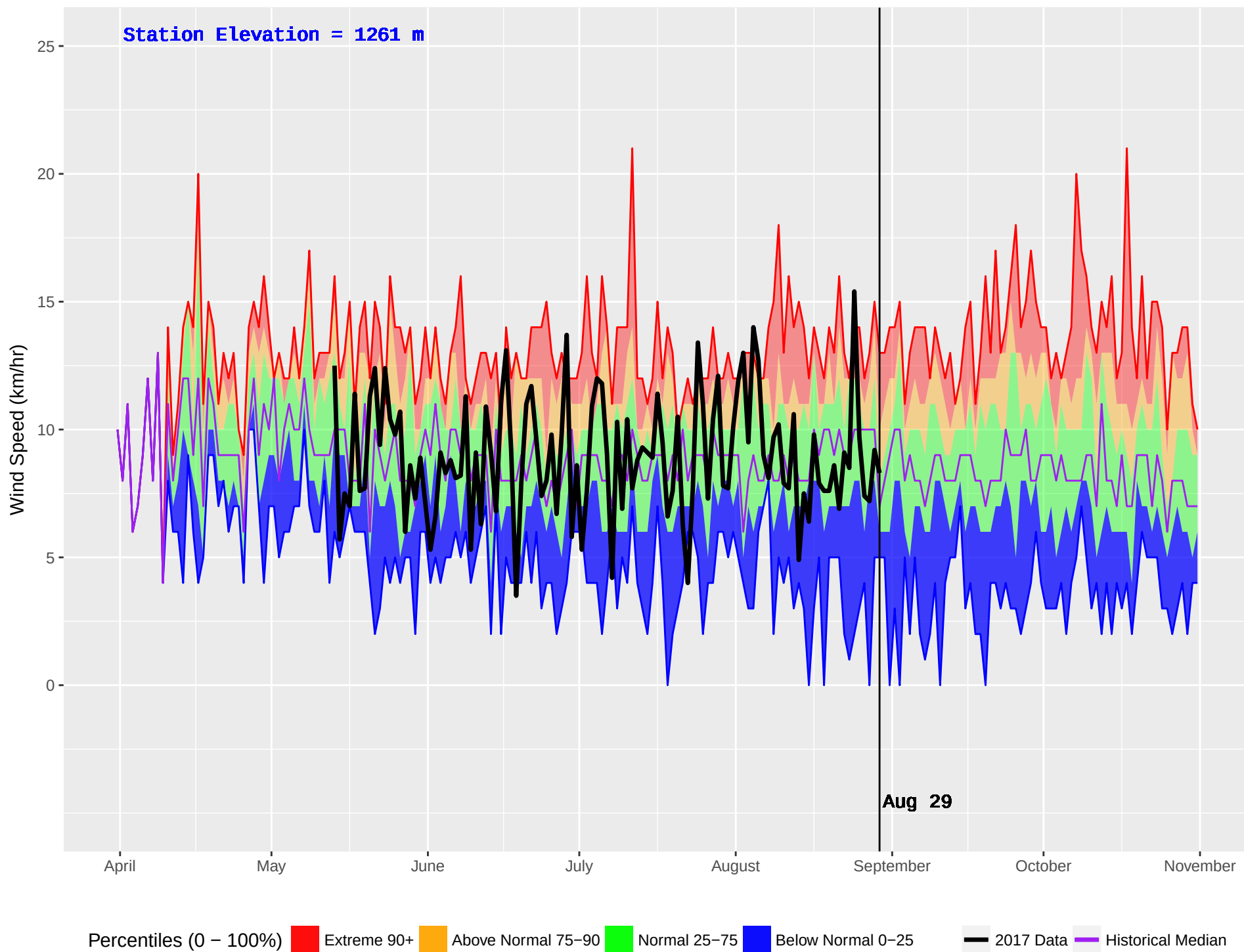
IDA BELL LAKE 3 (876) : Historical (2004–2016) and Current (2017) Noon Wind Speed
